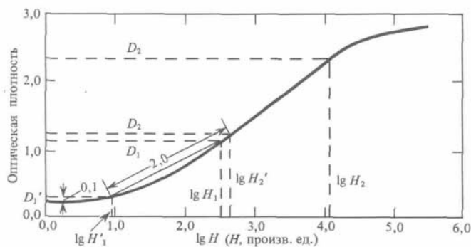
Рис. 8.6. Определение величин \gamma и среднего градиента 11 H Asher, Photographic Principles & Practices, Garden City, N Y Amphoto, 197 11 , p 200 2 > Kodak Professional Black-and-White Films, p 13
