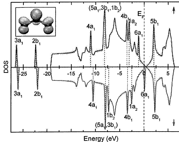
FIG. 5: (Color online) NO 2 on graphene. Inset: HOMO and LUMO of NO 2 (the N atom is blue and the O atom is red). Main panel: spin-polarised DOS of NO 2 on graphene.
