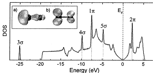
FIG. 4: (Color online) CO on graphene. Inset: (a) the HOMO and (b) the LUMO of CO (the C atom is black and the O atom is red). Main panel: DOS of CO on graphene.
