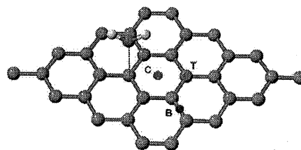
FIG. 1: (Color online) \text{H}_2\text{O} on graphene. 4 \times 4 supercell of graphene with adsorbed \text{H}_2\text{O} molecule.
