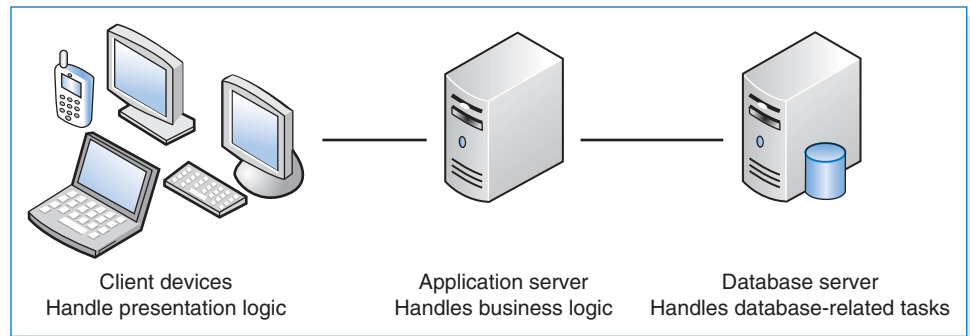
FIGURE 8-2 Three-Tiered Client–Server Architecture
