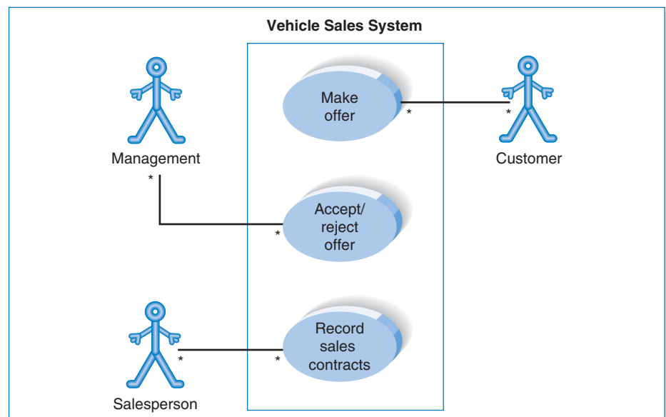
FIGURE 14-10 Use Case Diagram for Vehicle Sales System
