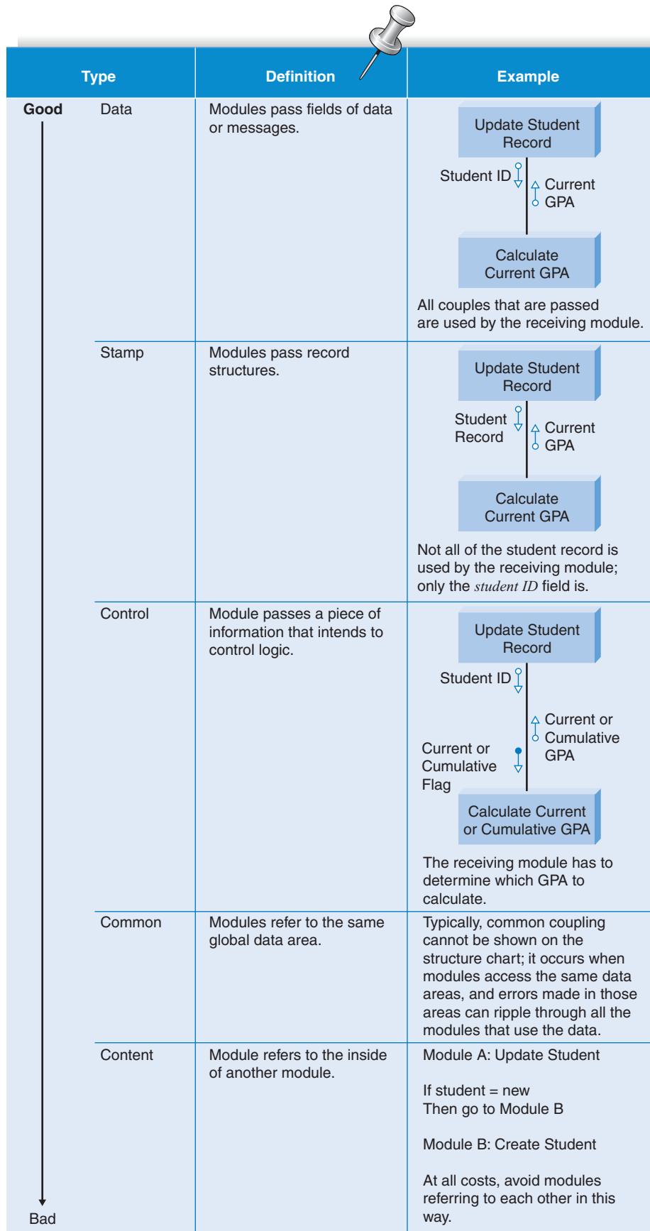
FIGURE 10-16 Types of Coupling (GPA = grade-point average)
