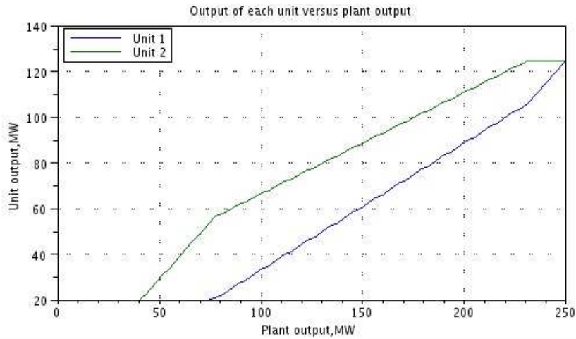
Figure 7.1: Incremental cost and load sharing
