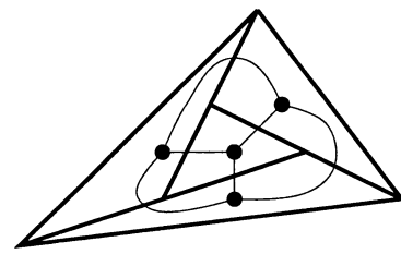
f(2) \geq 4
