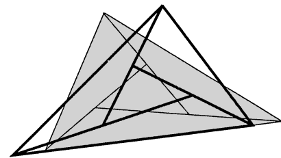
f(3) \geq 8
