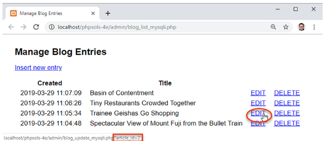
Figure 15-2. The EDIT and DELETE links contain the record's primary key in a query string
