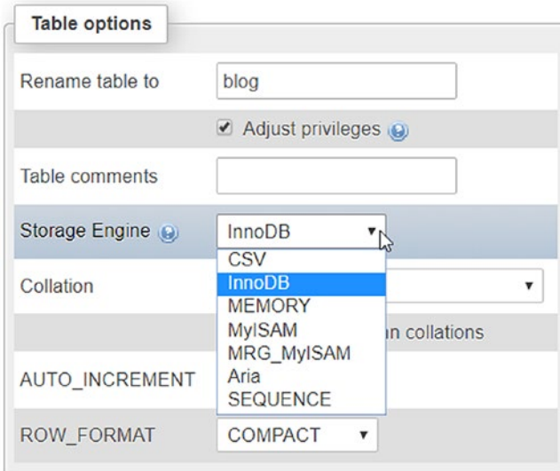
Figure 18-4. The available storage engines are listed in the Table options
