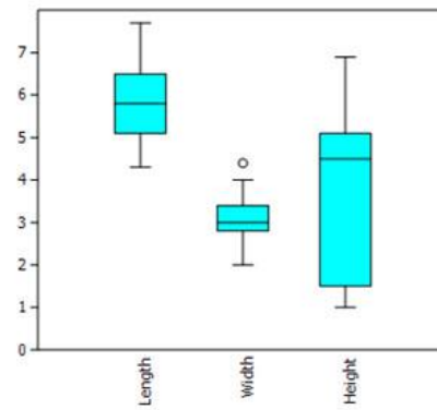
Box plot
