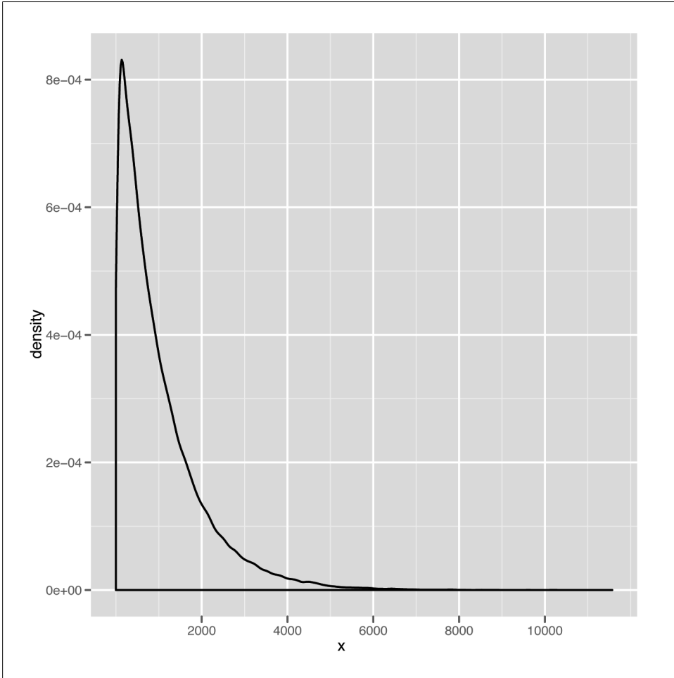
Figure 2-19. Skewed distribution
