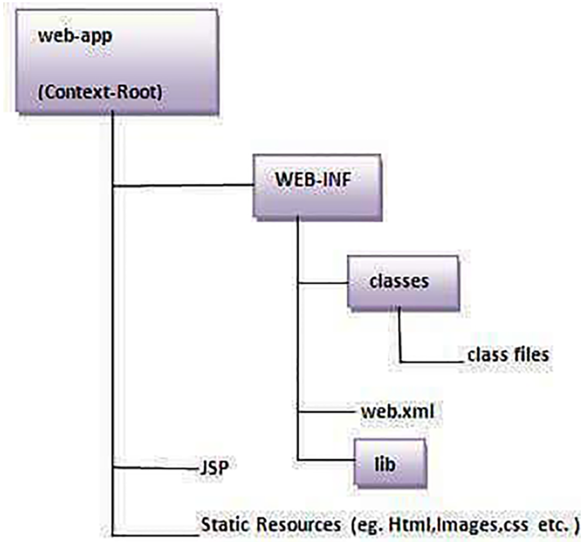
Figure 7.4: Directory Structure of the JSP page
