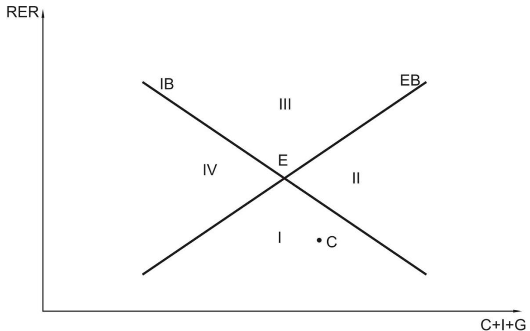
Figure 8.1. Swan diagram
