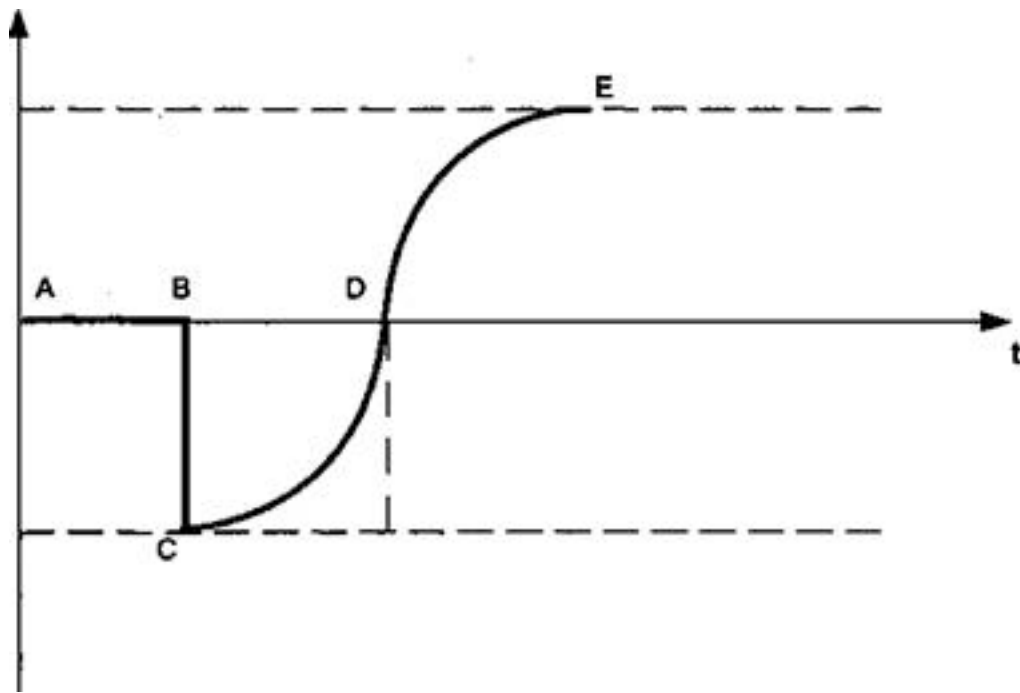
Figure 7.3. J-curve
